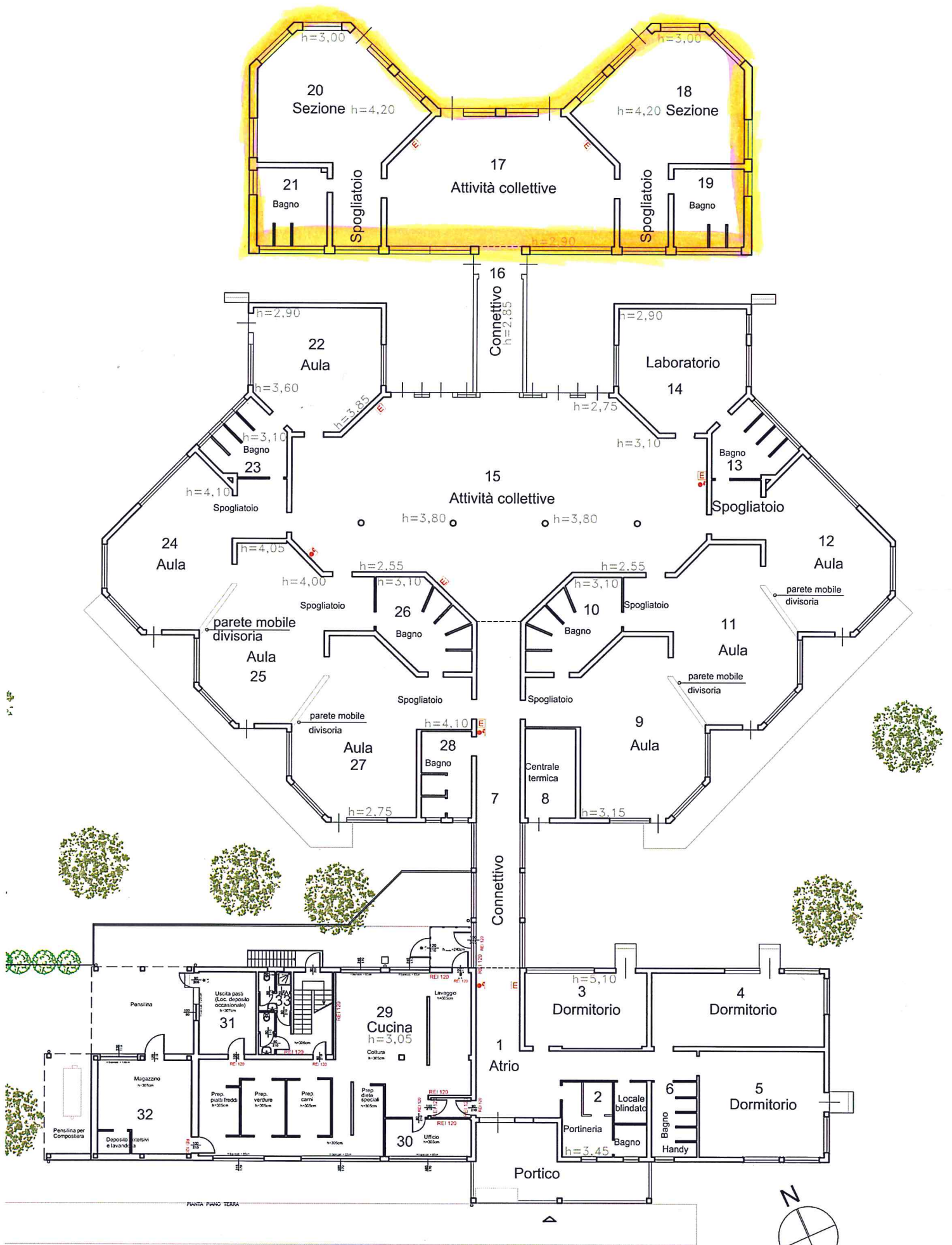
PIANO TERRA
